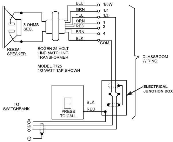
CA10A Wiring Schematic
