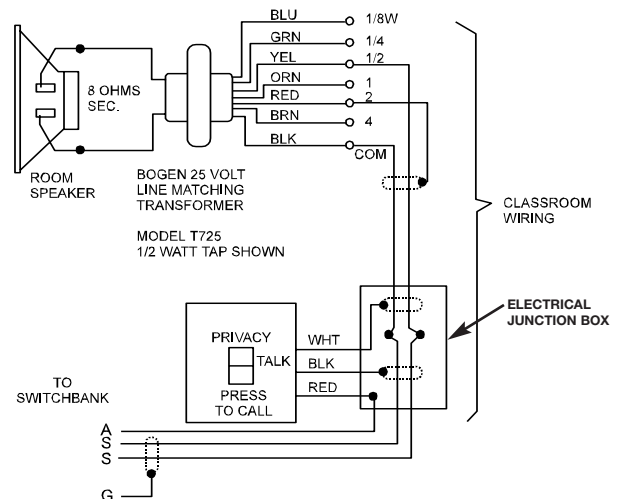
CA11A Wiring Schematic (with Privacy)
