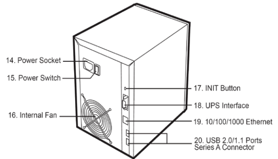
TeraStation Rear Panel
