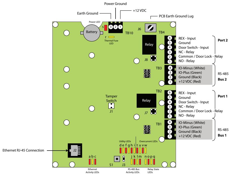
NXT-2D Installation Drawing
