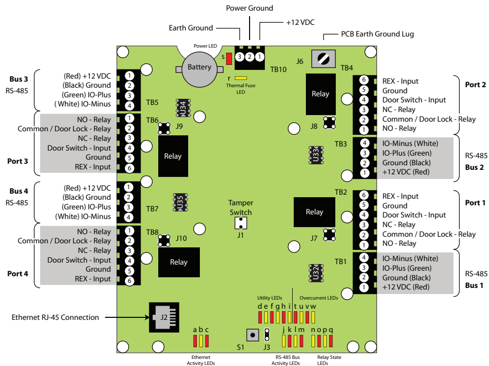
NXT-4D Installation Drawing
