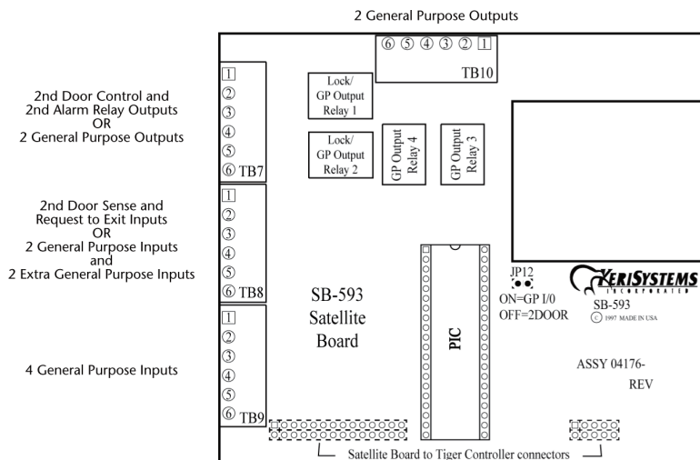
SB-593 Expansion Board
