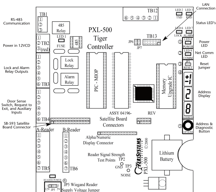
PXL-500 Tiger II Controller
