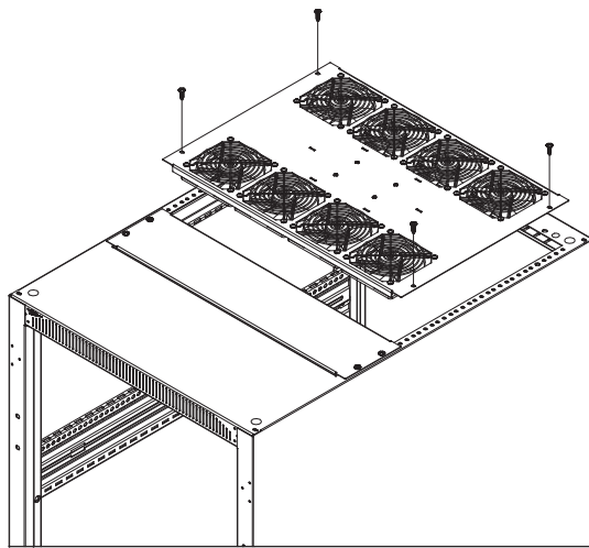
(I)BGR-552FT/(I)BGR-552FT-FC MODELS
