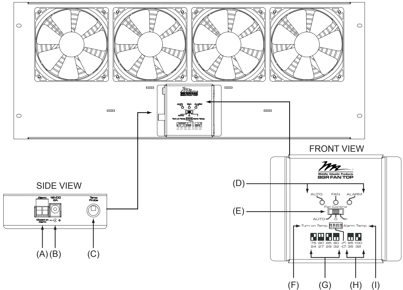
(I)BGR-276FT-FC SHOWN
