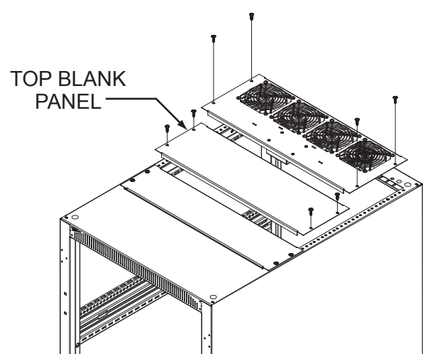
(I)BGR-276FT/(I)BGR-276FT-FC MODELS
