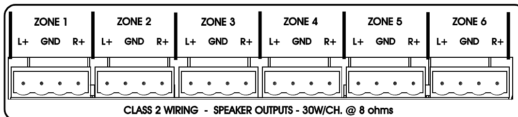
Figure 3-10: Speaker Connections
