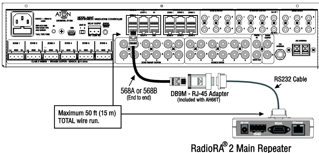
Figure 4-4: RadioRA 2 Connections
