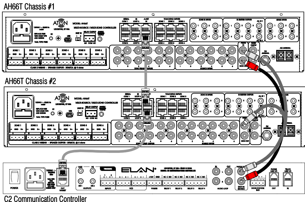
Figure 4-7: C2 Connections
