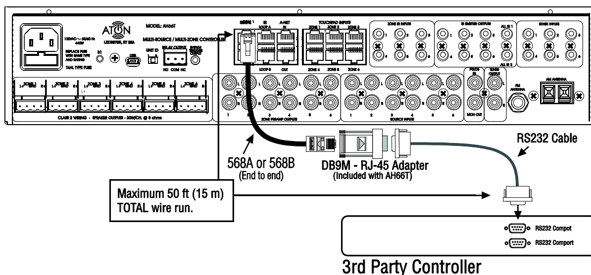
Figure 4-6: RS-232 Connection
