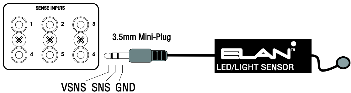
Figure 3-6: Sense Inputs
